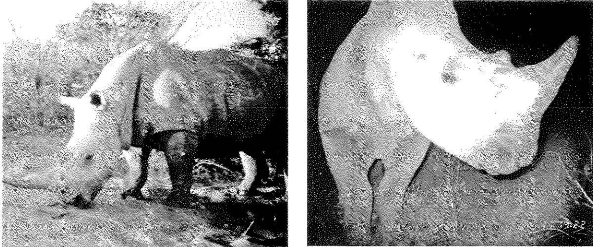
Figure 2. Photographs of white rhinos taken within the Waterberg Plateau Park using motion-sensor camera traps between June and October of 2006. Note the marked difference in horn size and shape between individuals.
